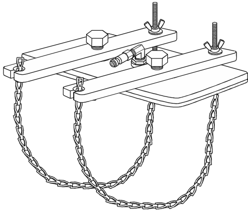
PF9003 Universal adaptor, large rectangular
