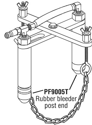
PF9005 GM bypass adaptor (Direct contact adaptor)
