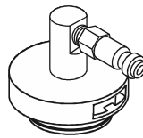
PF9033 Isuzu Cabover adaptor (pipe thread)
